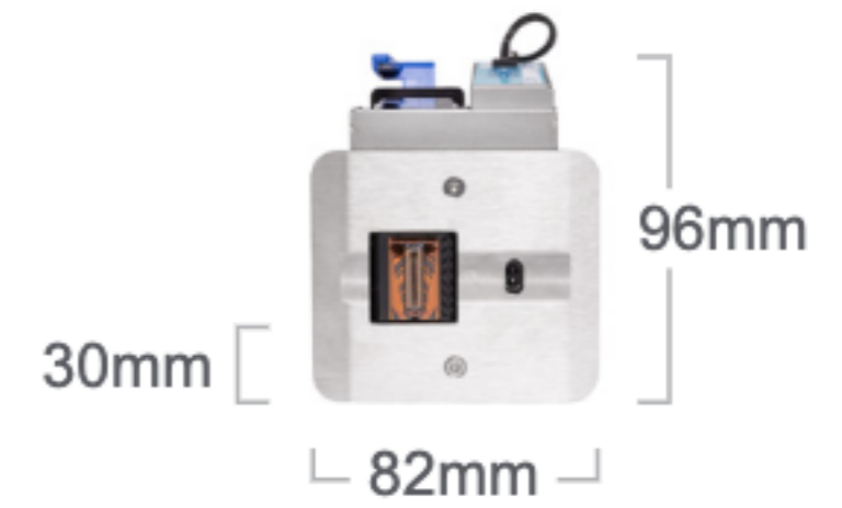
LX PRINTHEAD FRONT ELEVATION
