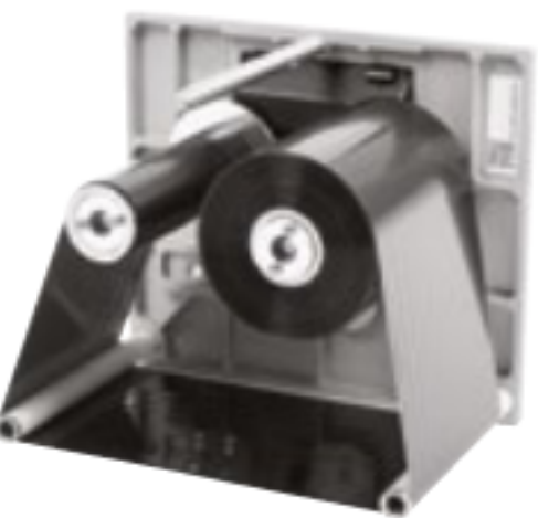
RIBBON CASSETTE
